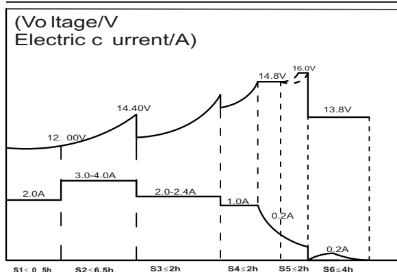
Charging characteristic
